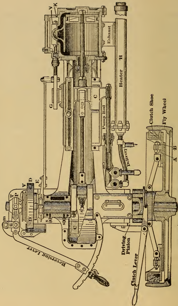
Ericsson 'Disengaging Clutch' FIG. 5.
